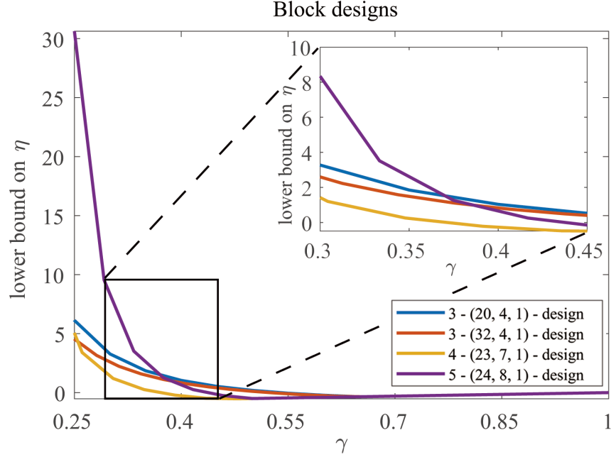
Fig. 3. The lower bound on \eta by Theorem 2, versus the corrupted fraction \gamma , when \mu = (r - 1)/k . All four designs shown in this figure have explicit constructions [32]. \eta < 0 if the custody scheme is not secure for corresponding \gamma .
