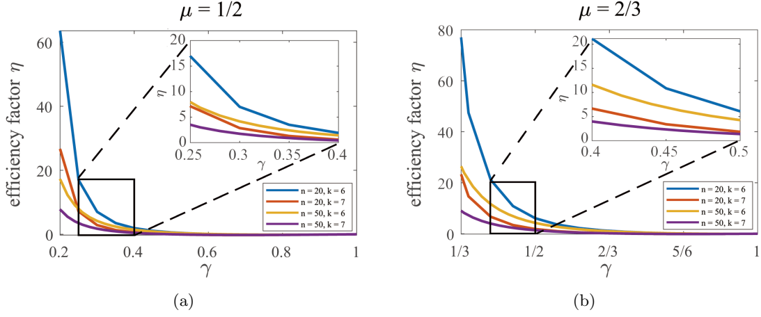
Fig. 1. The efficiency factor \eta versus the corrupted fraction \gamma for \mathcal{A}_{all} as in Construction 1. In particular, \eta < \gamma if the custody scheme is not secure for corresponding \gamma .
