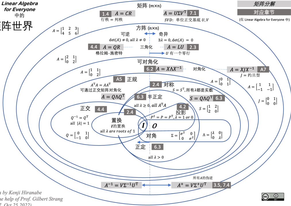
Figure 19: 矩阵世界
